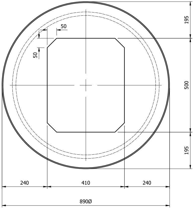
50mm GRADE RING
