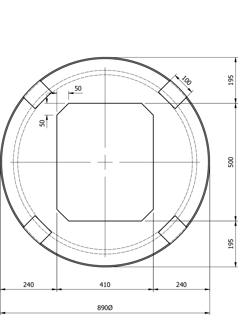
100mm GRADE RING
