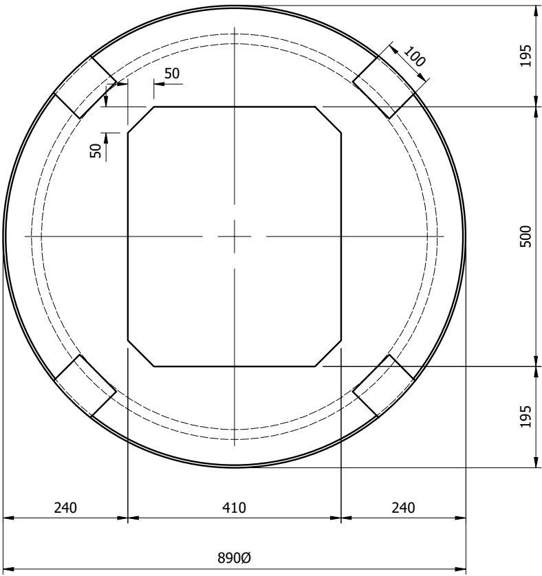
75mm GRADE RING
