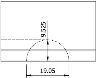
DETAIL A GROOVE DETAIL SCALE 1:1
